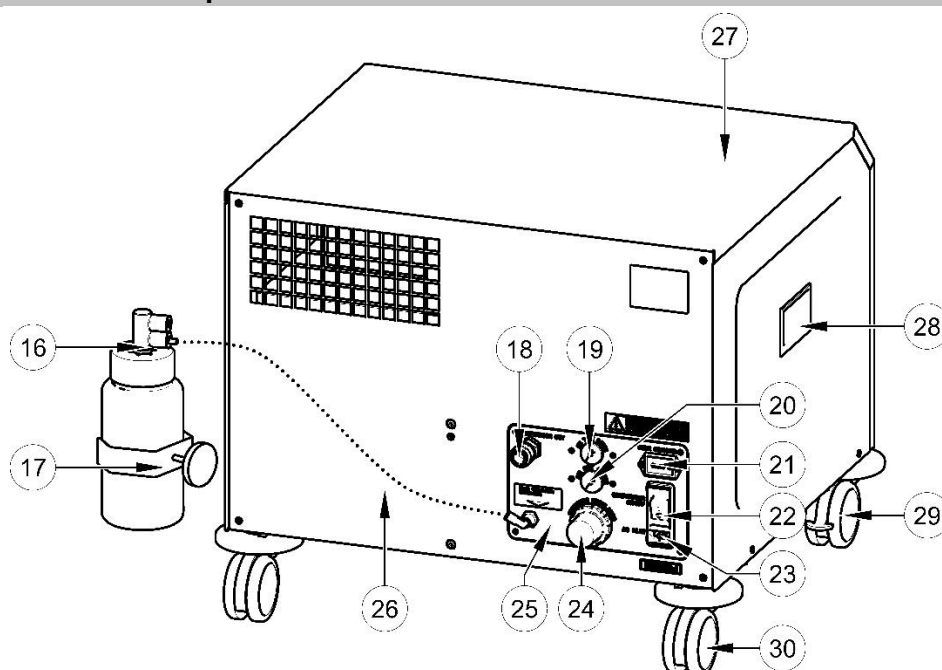
Obr. 1: DK50-10S/M – Kompresor
