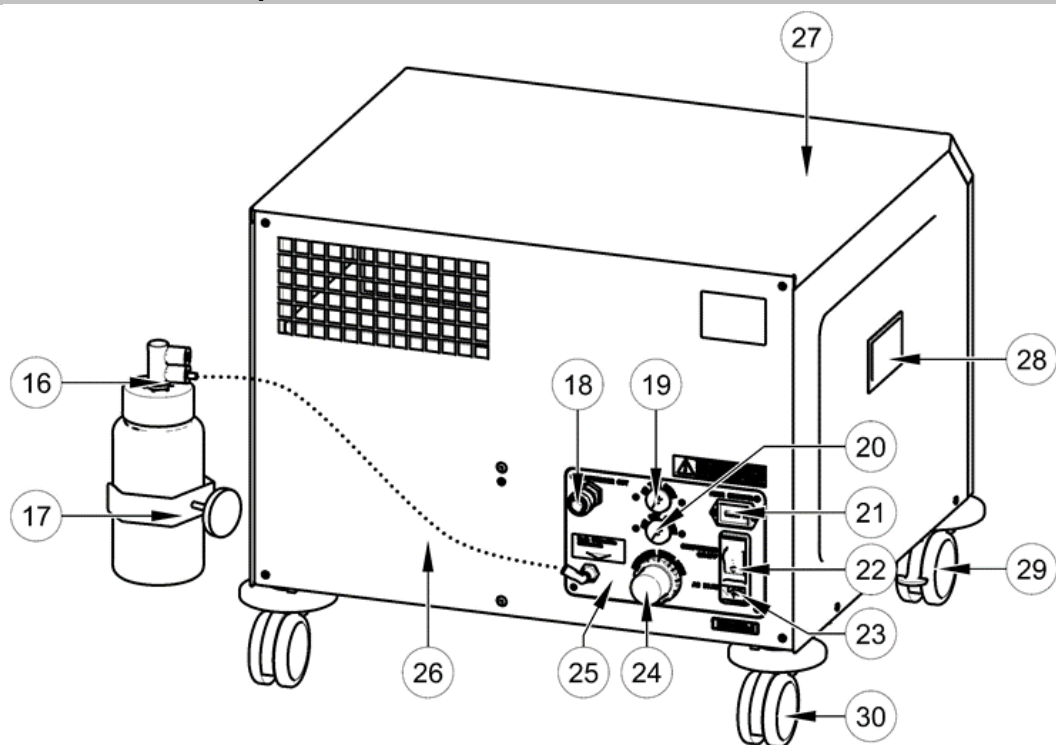
Fig. 1: DK50-10S/M – Compressor
