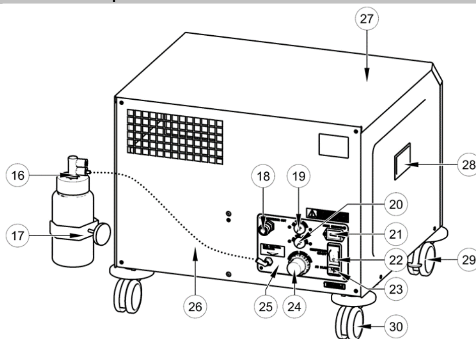
Abb. 1: DK50-10S/M – Kompressor
