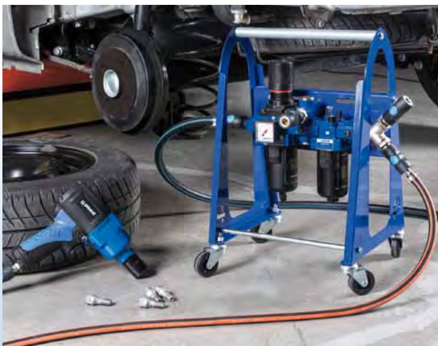
Air treatment and distribution assembly
